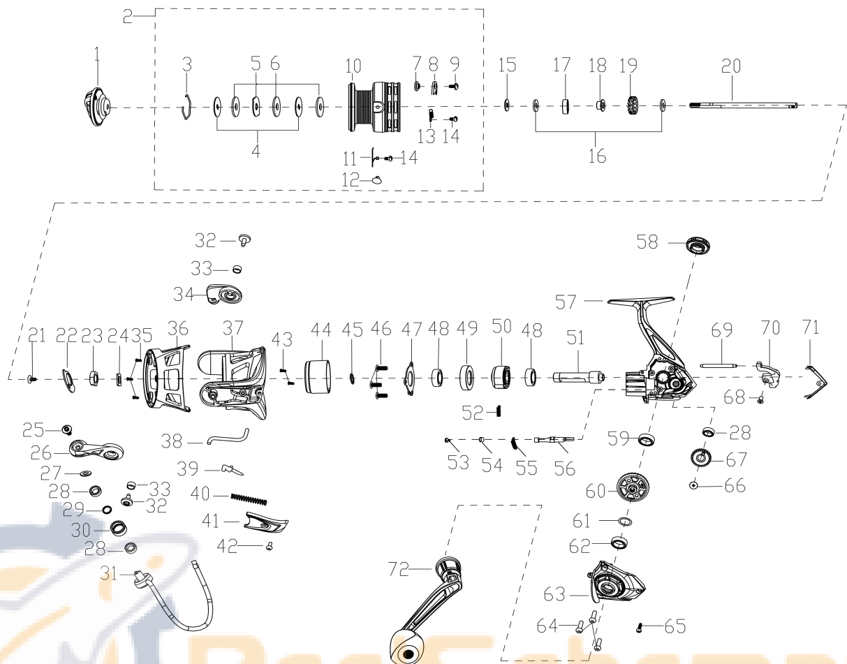
PARTS LIST OF CS4-3000
